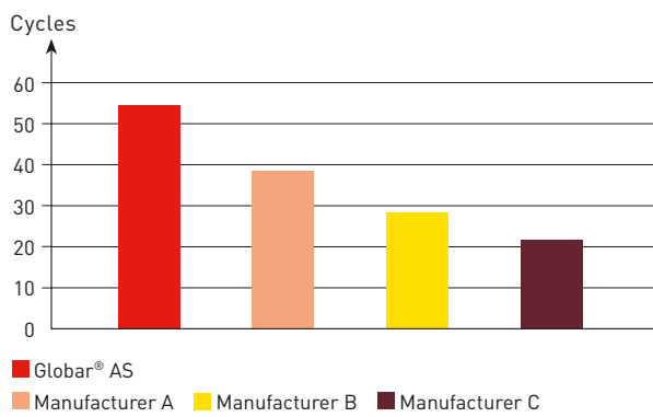
Cyclic test: Globar® AS vs. other manufacturers' elements. 100 hour cycles at 1425°C (2600°F).
